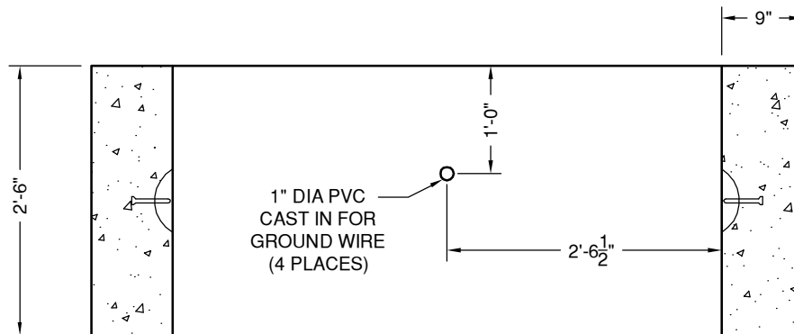
SECTION VIEW
