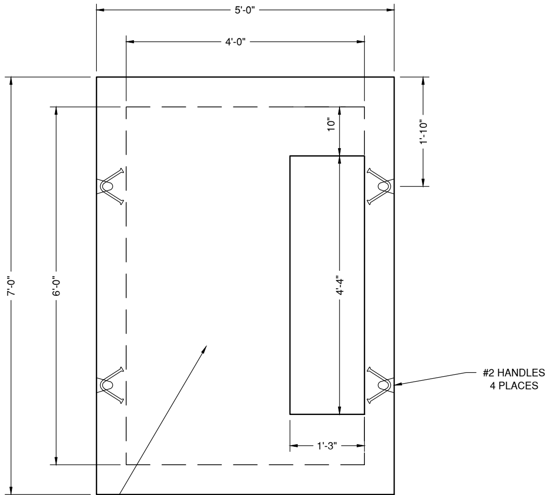
PLAN VIEW
