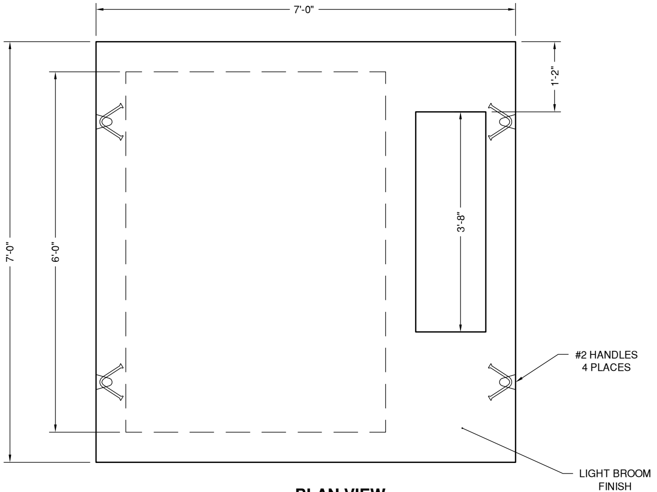
PLAN VIEW
