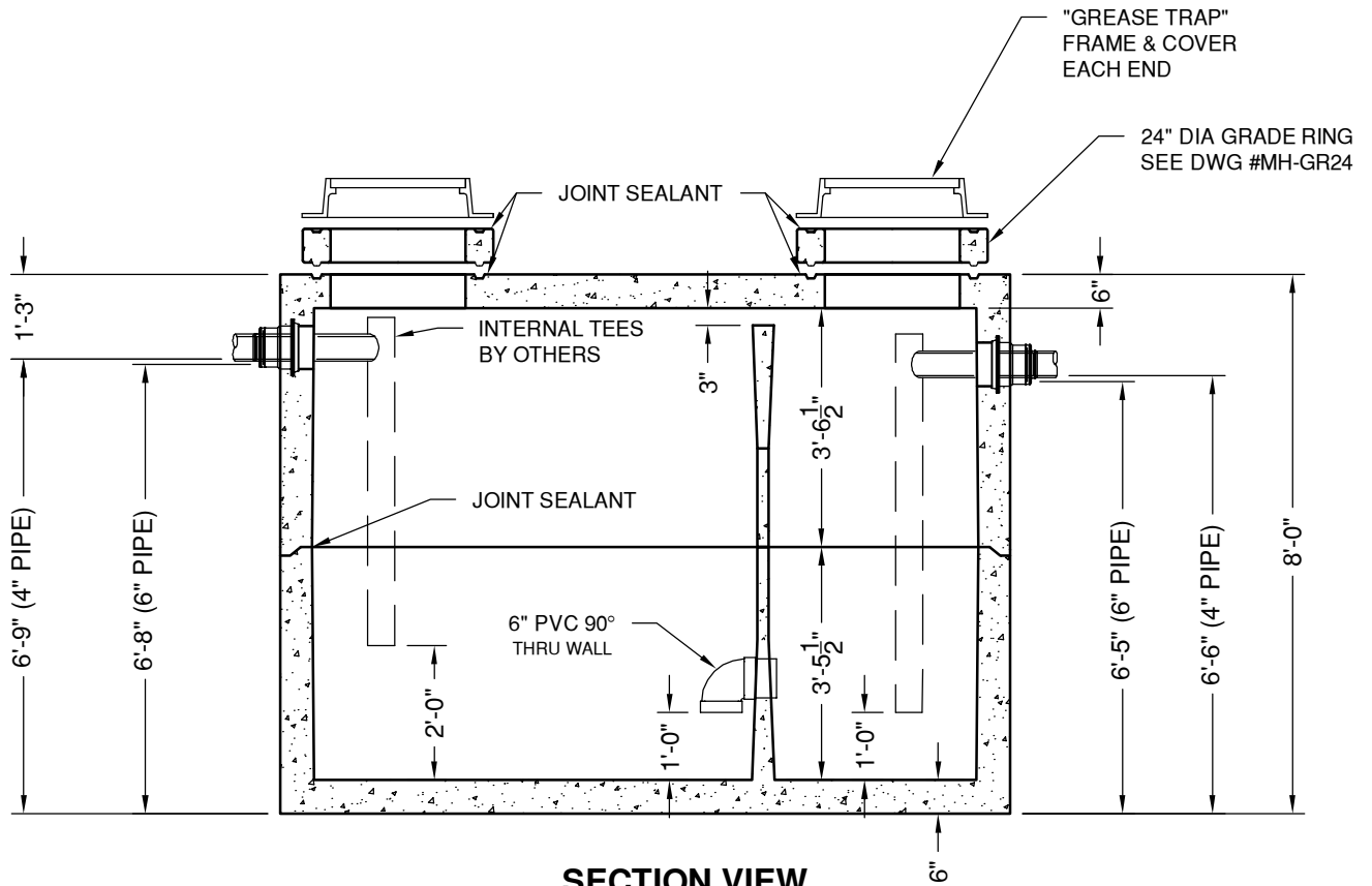
SECTION VIEW
