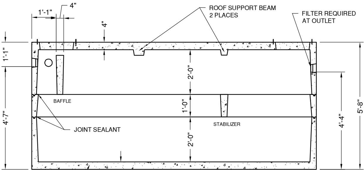
SECTION VIEW
