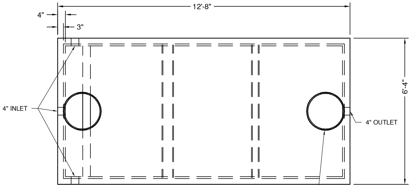
PLAN VIEW
