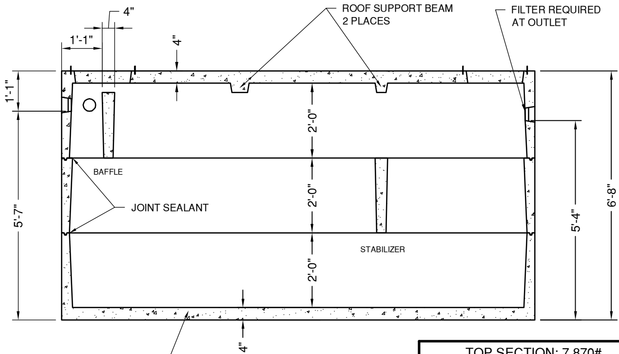
SECTION VIEW
