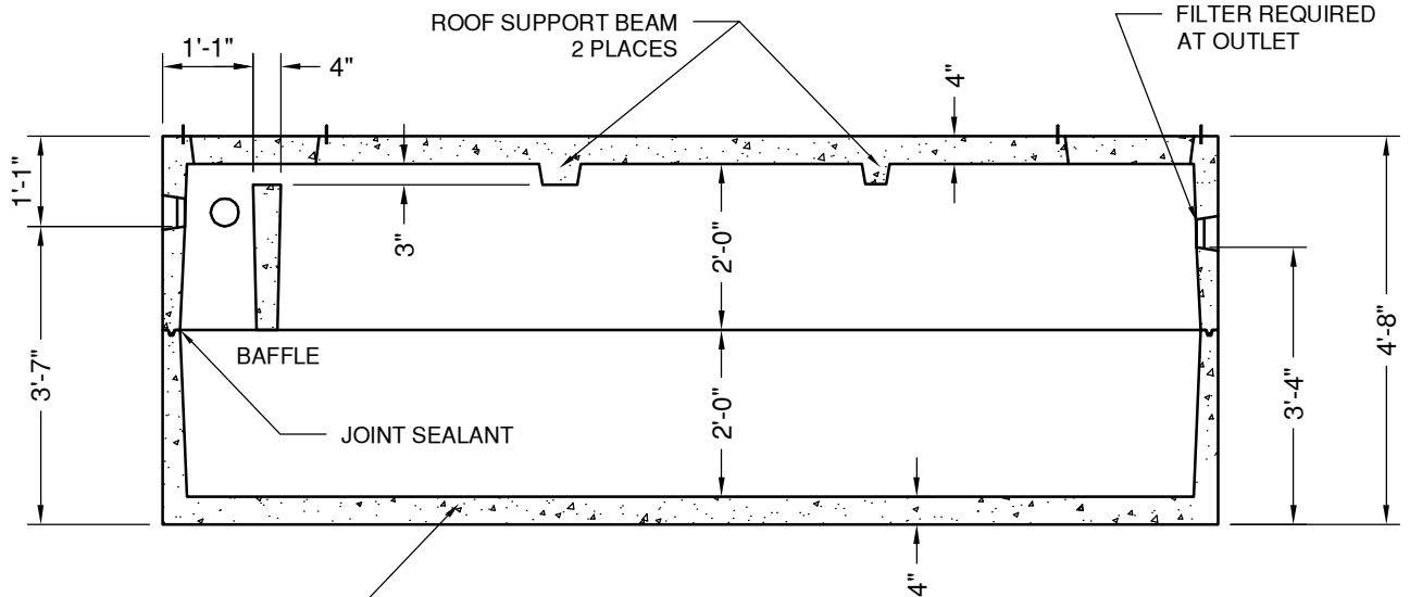
SECTION VIEW
