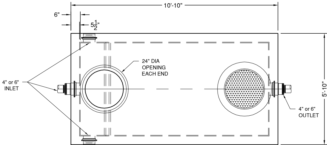
PLAN VIEW
