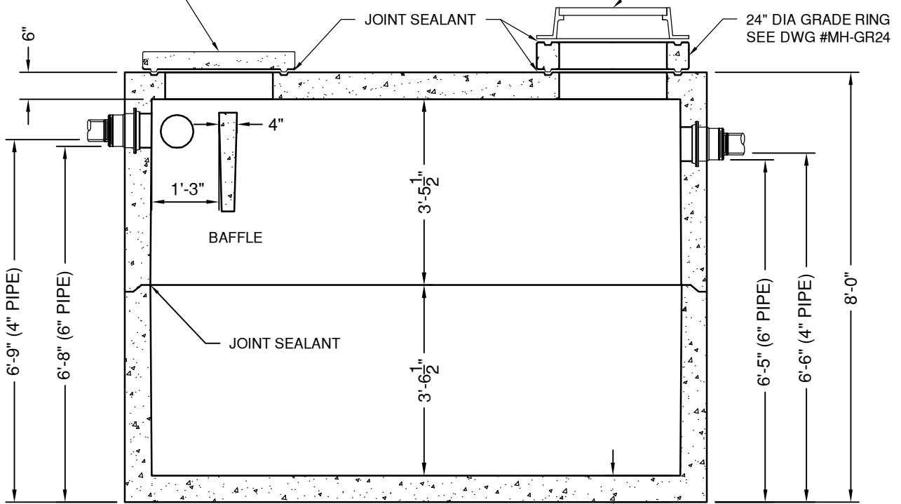
SECTION VIEW
