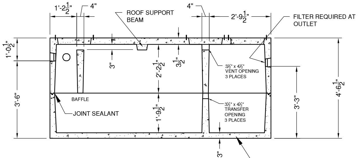
SECTION VIEW
