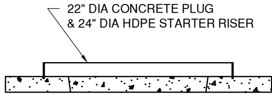
LID w/RISER - SECTION VIEW
