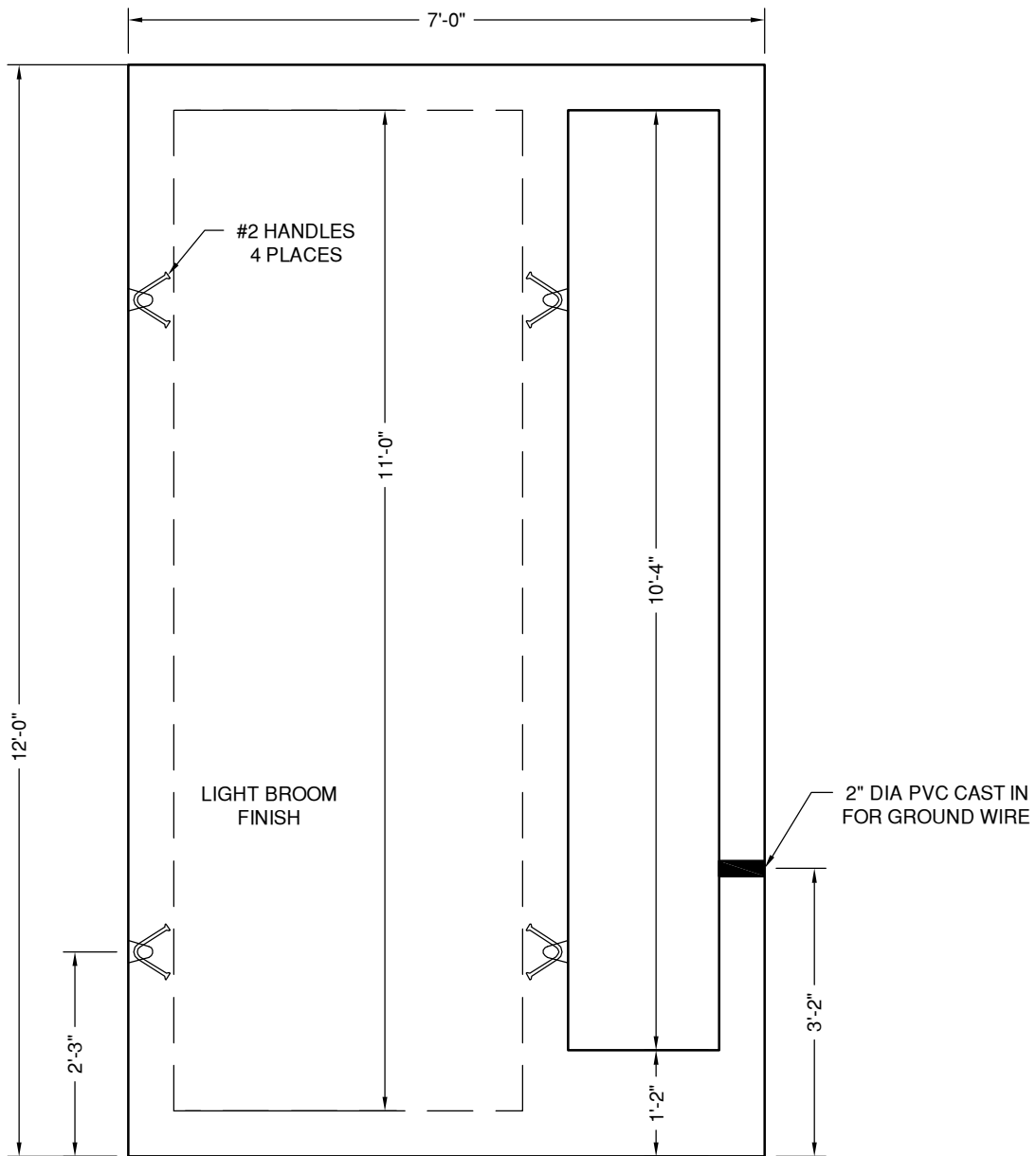
PLAN VIEW
