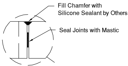
JOINT DETAIL
