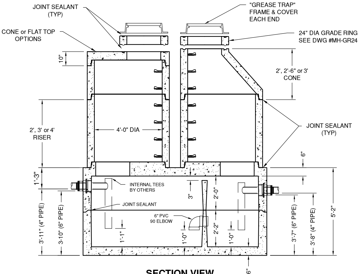
SECTION VIEW
